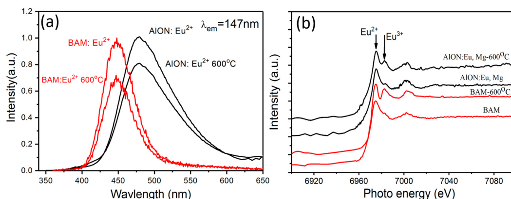
Figure 6. Emission intensity (a) and \text{Eu L}_3 -edge X-ray absorption near edge structure (XANES) spectra (b) of AION:Eu, Mg and \text{BaMgAl}_{10}\text{O}_{17}:\text{Eu}^{2+} phosphors before and after annealing at 600 °C for 1 h in air.
