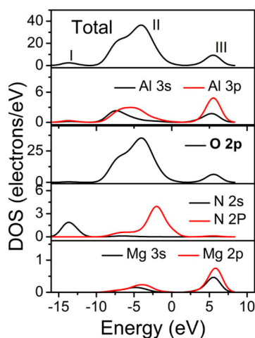
Figure 5. The total and the atom-resolved partial density of states (PDOS) for all the different atoms in \text{Al}_{21}\text{Mg}_2\text{O}_{29}\text{N}_3 .
